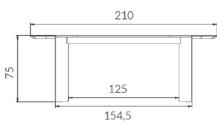
cm 210x95xH75
