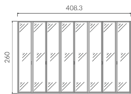
cm 408.3x60.3xH260
