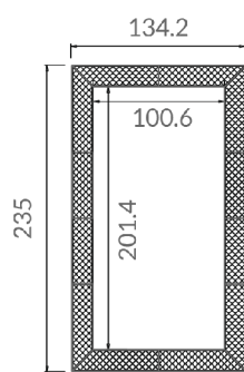
cm 134.2x13xH235
