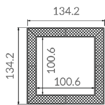
cm 134.2x13xH134.2
