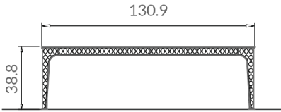
cm 130.9x13.9xH38.8
