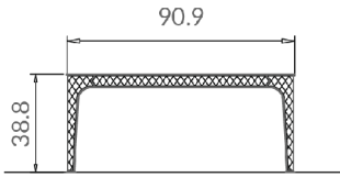
cm 90.9x90.9xH38.8
