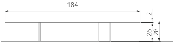
cm 184x70xH28
