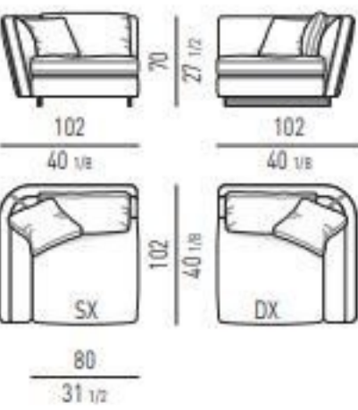
ELEMENTO TERMINALE/ANGOLARE LOW CM 102 CORNER ELEMENT WITH ARMREST LOW CM 102
