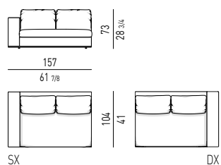
ELEMENTO TERMINALE CM 157 ELEMENT WITH 1 ARMREST CM 157
