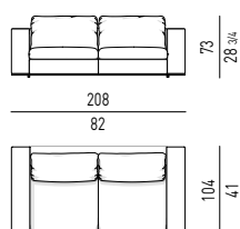
DIVANO CM 208 SOFA CM 208
