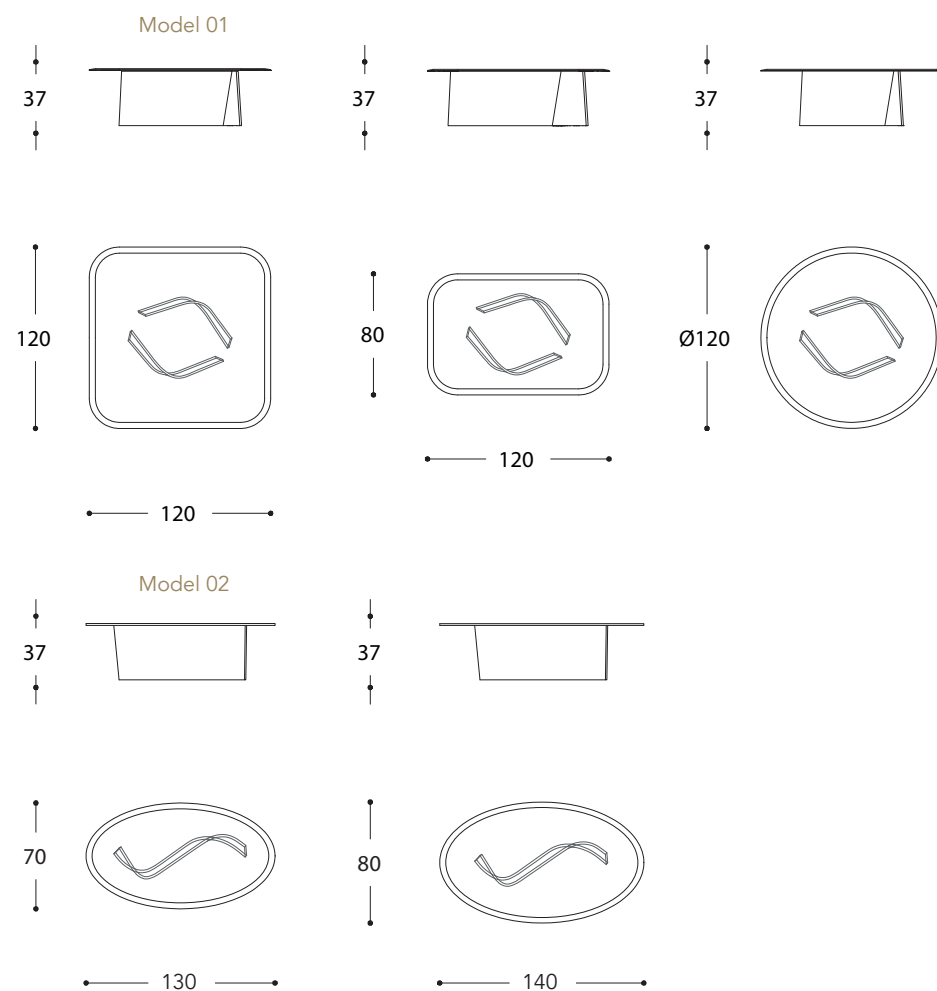
top detail
