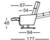
Recliner large, with plate foot
