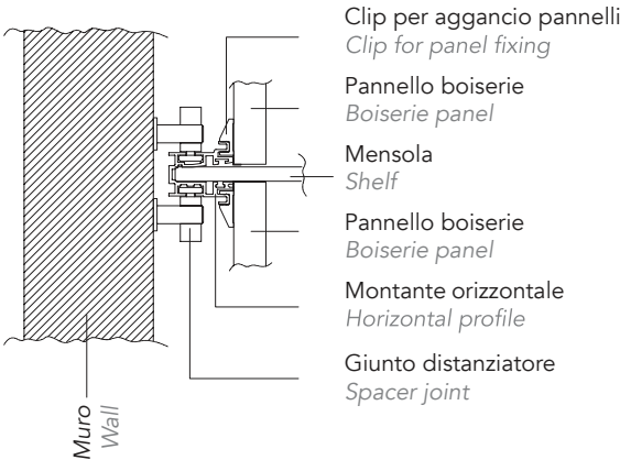
DETAIL 2 a) Aggancio a muro Wall mounting
