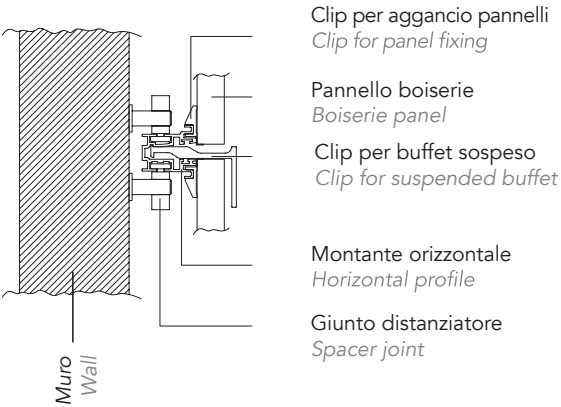
DETAIL 3 a) Aggancio a muro Wall mounting
