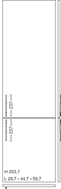
FRIGO - DISPENSA 1 ANTA COLUMN FRIDGE - CABINET
