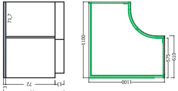
ANGOLO BASE 110 X 110 CORNER BASE UNIT
